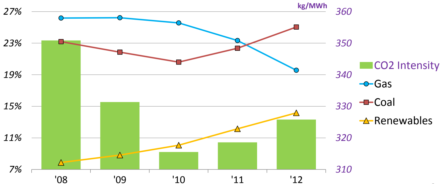
Generation and CO 2 Intensity in Power Sector of Western Europe 10
