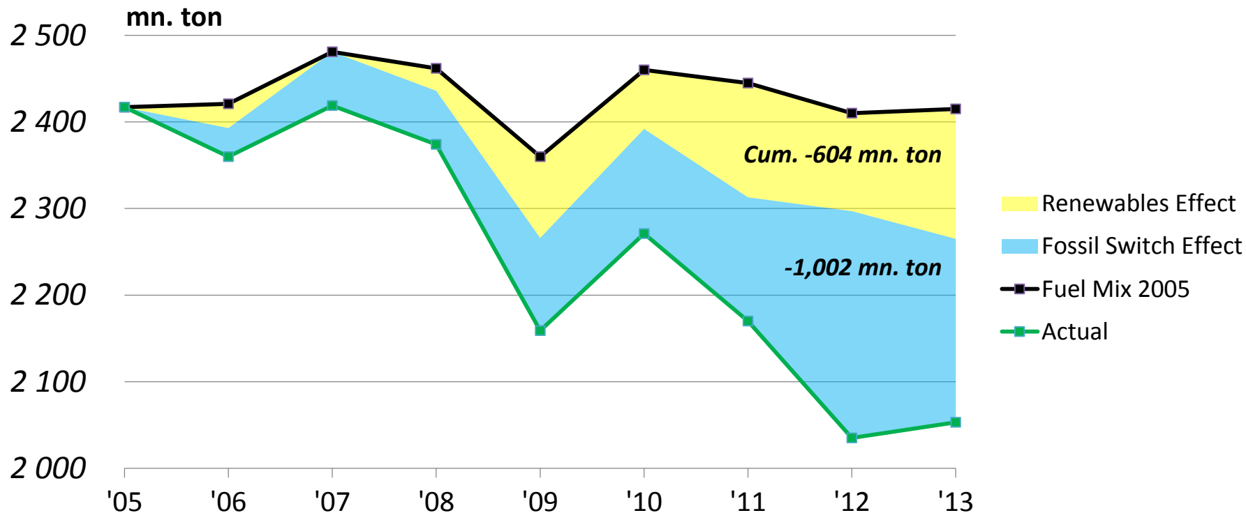
US Power Sector CO 2 Emissions: 2005 Case v. Actual
